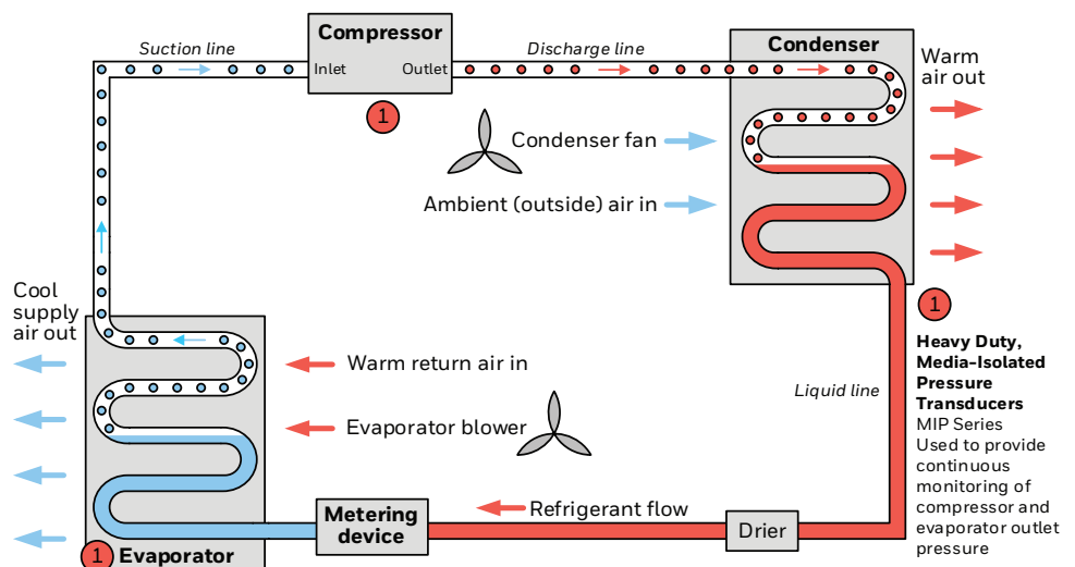
Figure 1. MIP Series Heavy-Duty Media-Isolated Pressure Transducers in Refrigeration Applications
